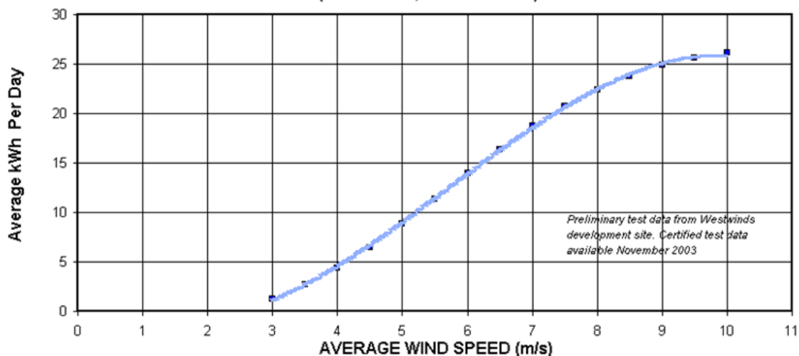
ESTIMATED OUTPUT IN kWh PER DAY FOR 3kW WIND TURBINE ( Sea level site, Weibull factor 2 )
